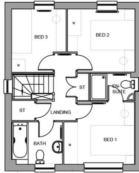
FIRST FLOOR PLAN Collaton
