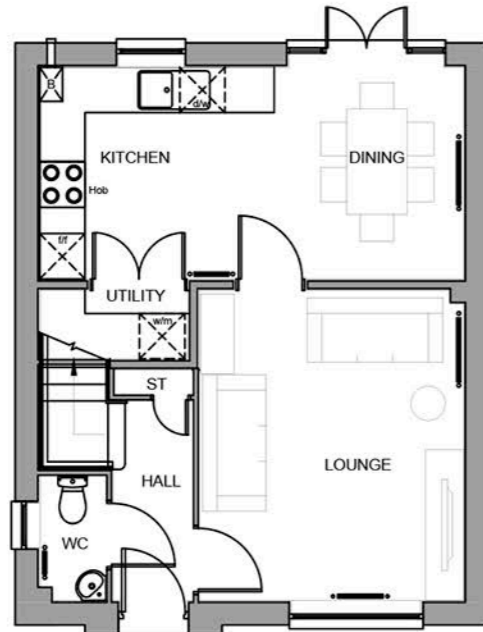
GROUND FLOOR PLAN Collaton
