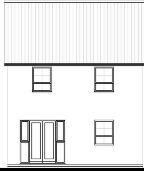
REAR ELEVATION Collaton
